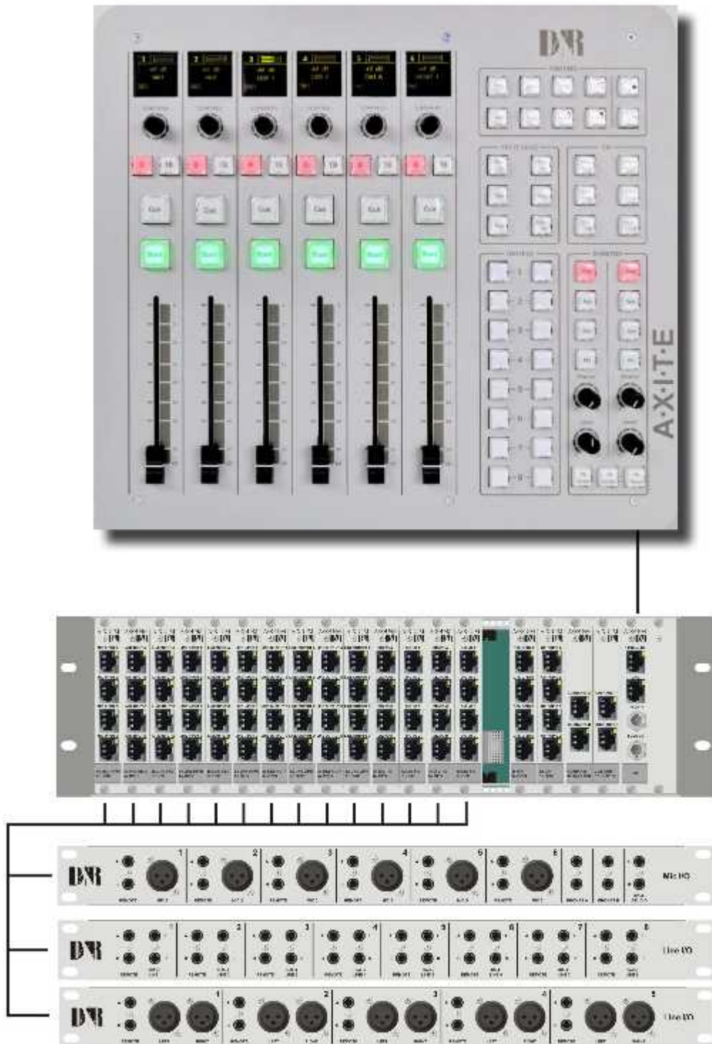
6 fader set up example with Rack One and three break-out panels.
